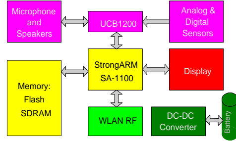
Figure 2: SmartBadge
